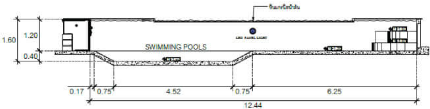
SECTION - A 1:100
